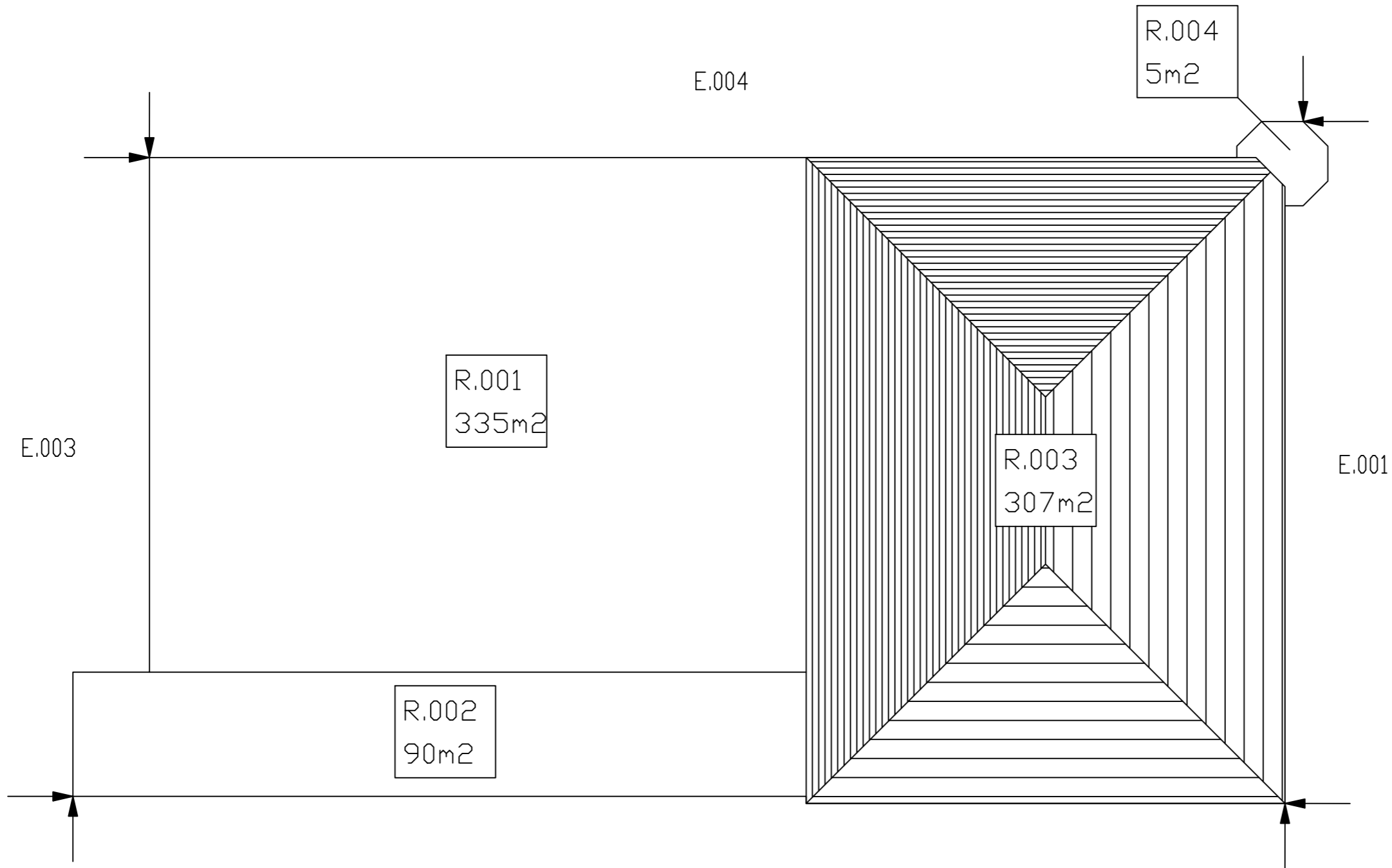
E.002 MAIN BUILDING - ROOF PLAN
