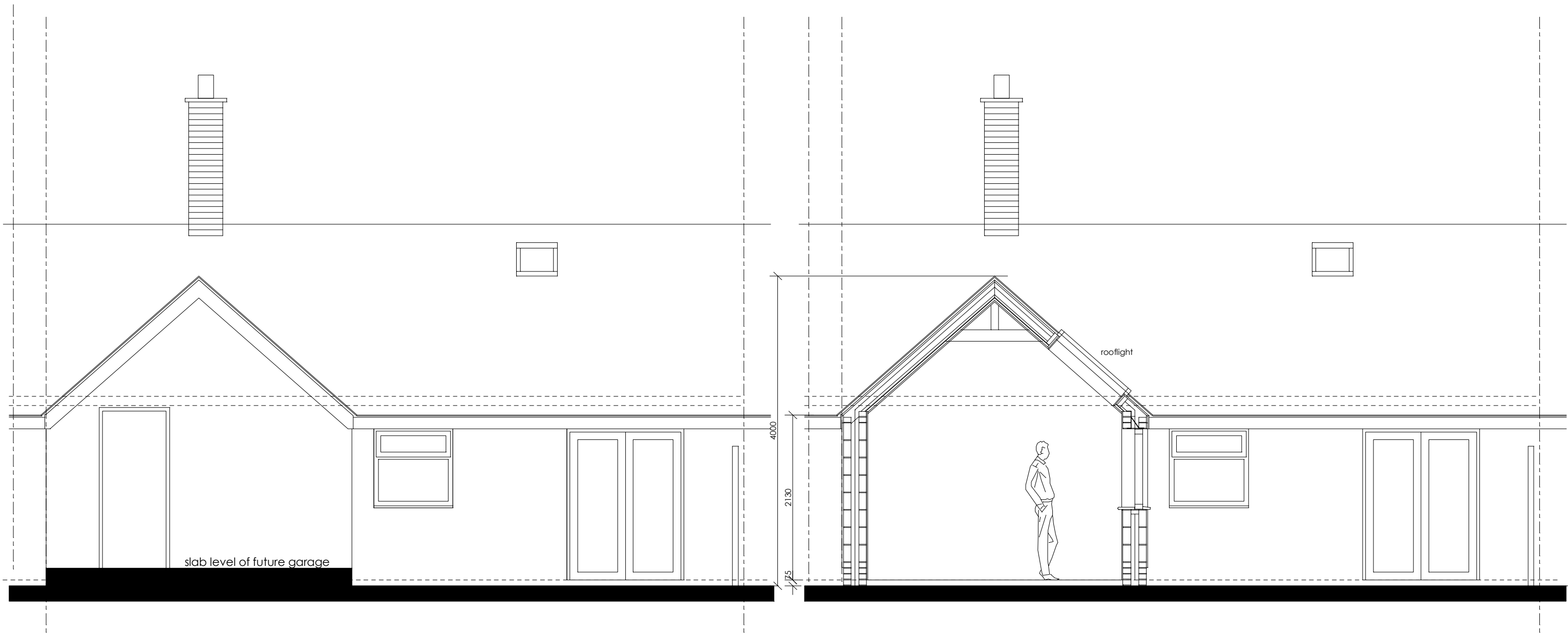
End elevation without garage
