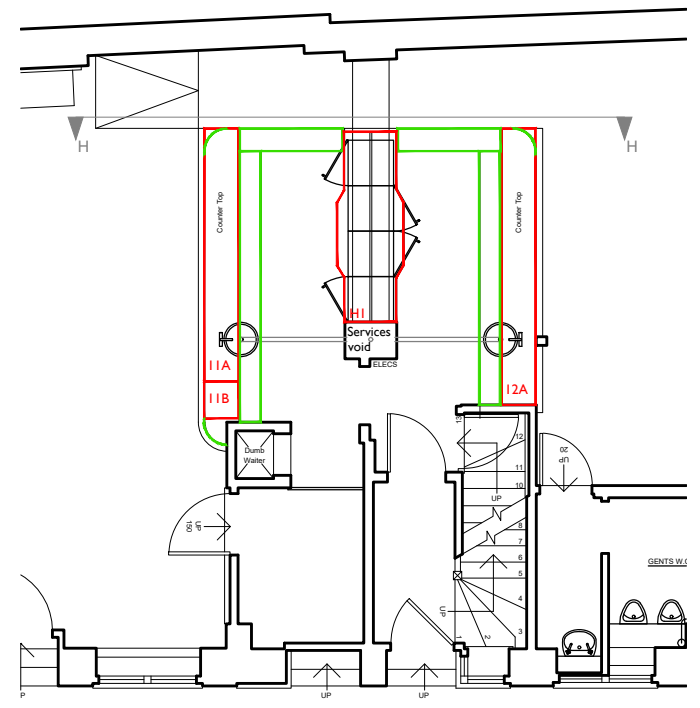
2 2018 KEY PLAN 1:100 @ A3
