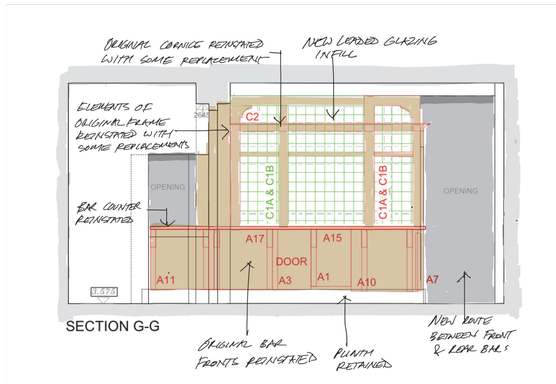
1 Proposed Section G 2017 1:50 @ A3
