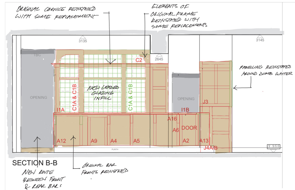
1 Proposed Section B 2012 1:50 @ A3
