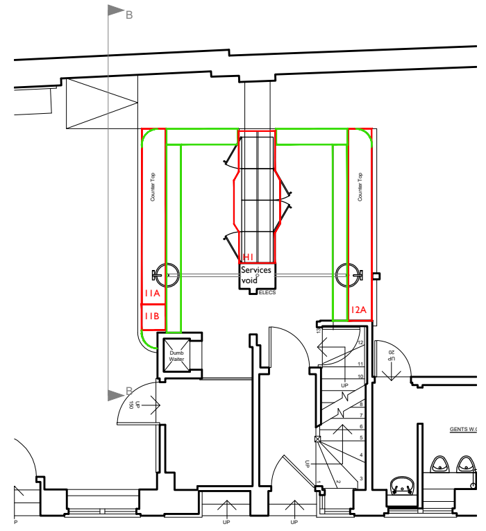
2 KEY PLAN 2012 1:100 @ A3
