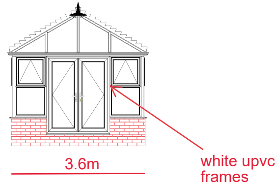
FRONT ELEVATION Scale 1:100
