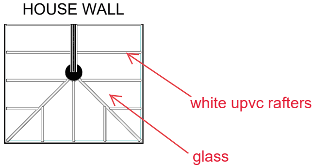
PLAN VIEW Scale 1:100
