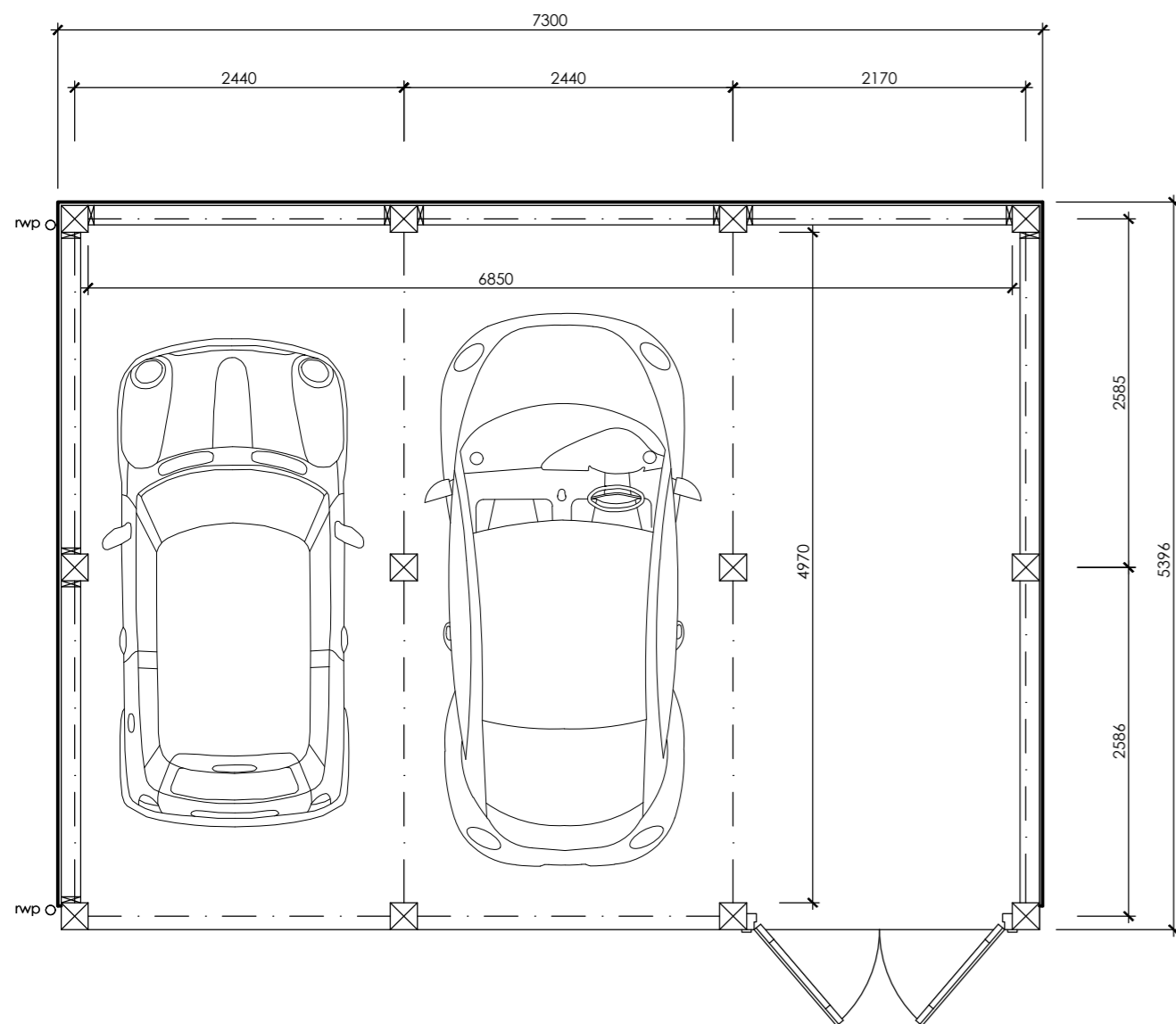
GROUND FLOOR PLAN - EXTERNAL PERIMETER = 39.400 sq.m
