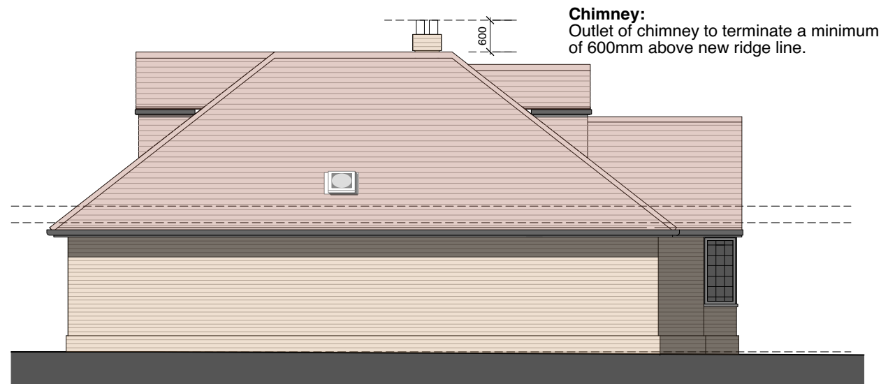
North Elevation
