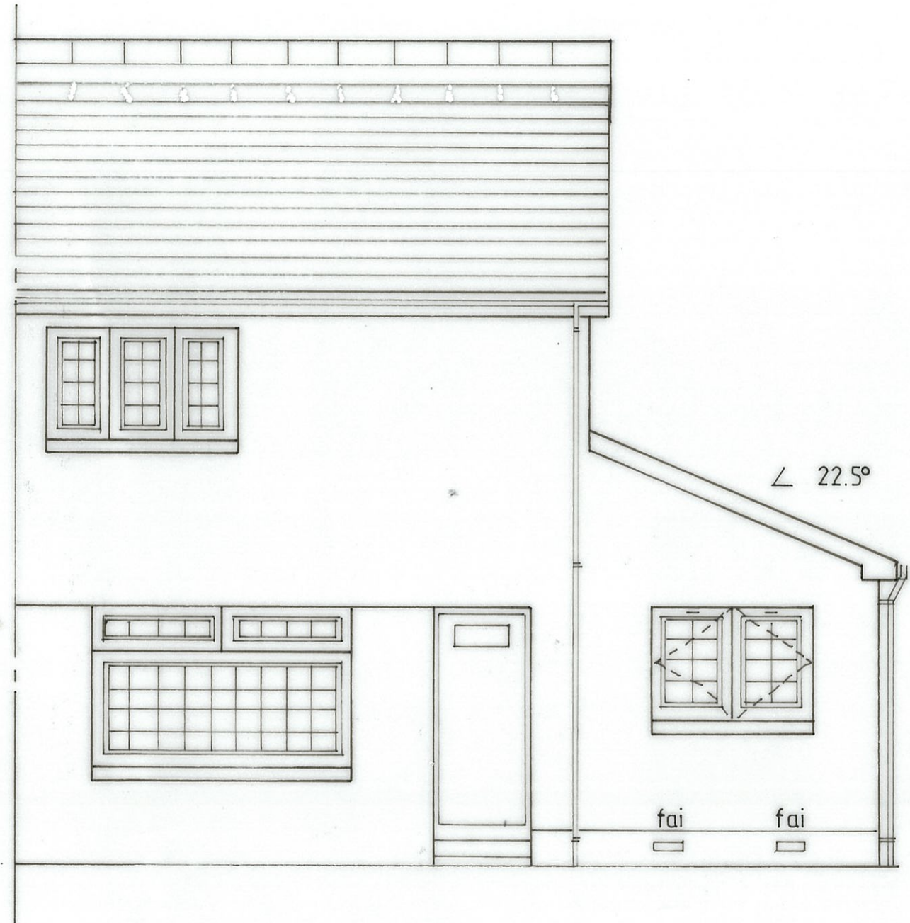
PROPOSED FRONT ELEVATION 1:50
