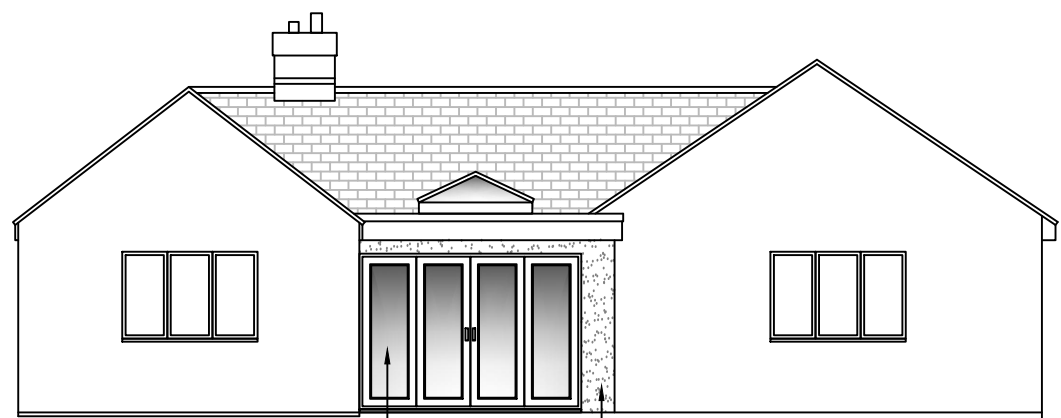
REAR ELEVATION
