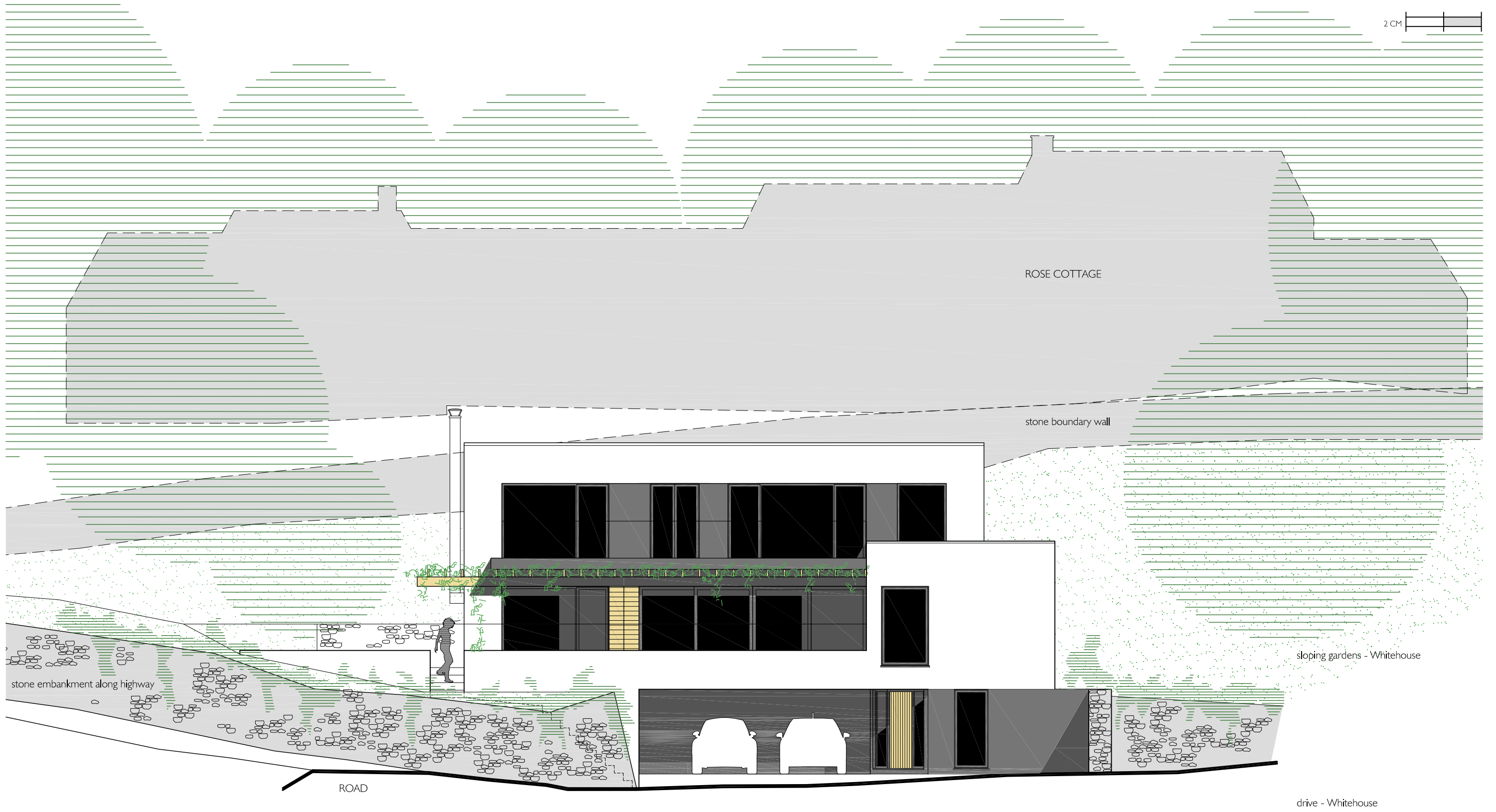
SOUTH ELEVATION
