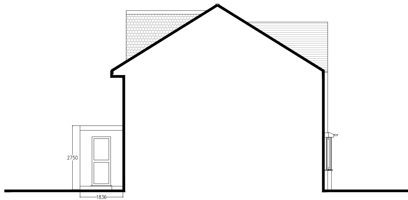
East Elevation
