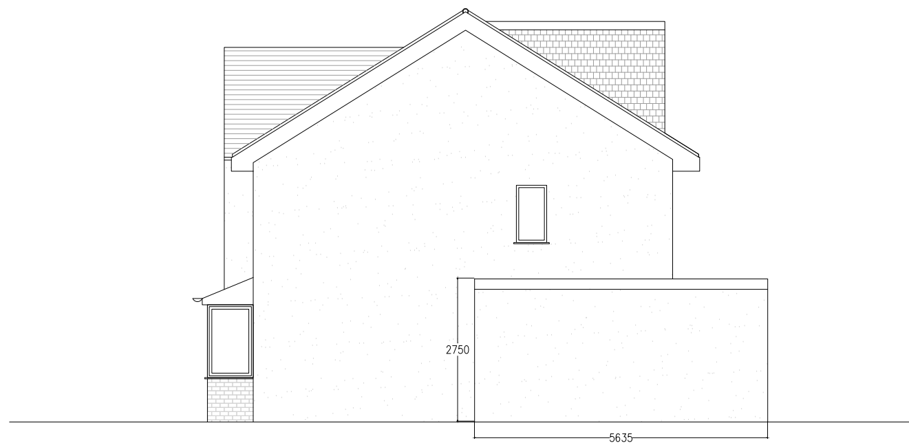
West Elevation
