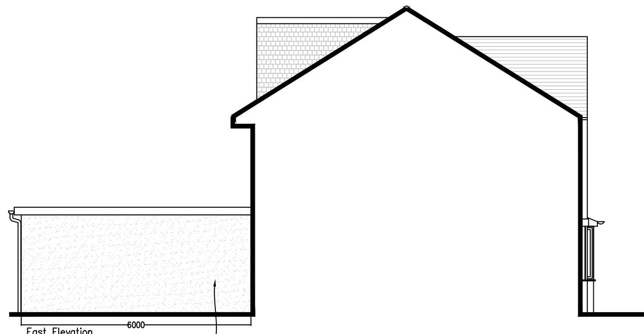
East Elevation
