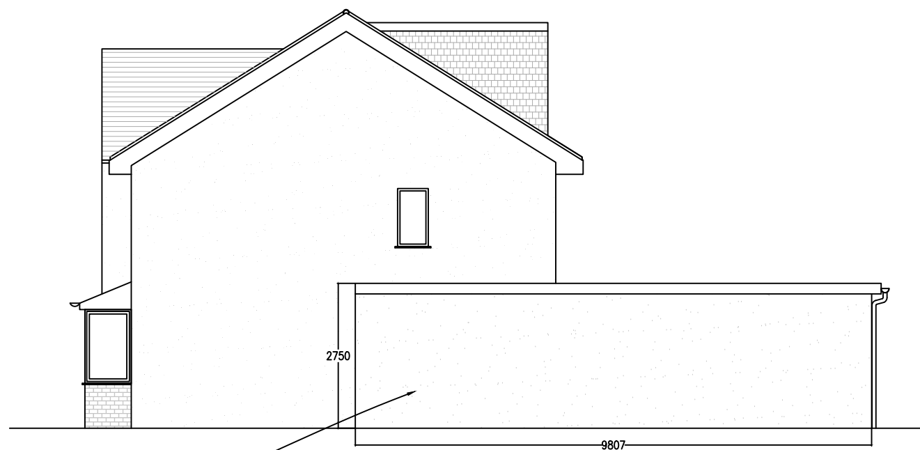
West Elevation
