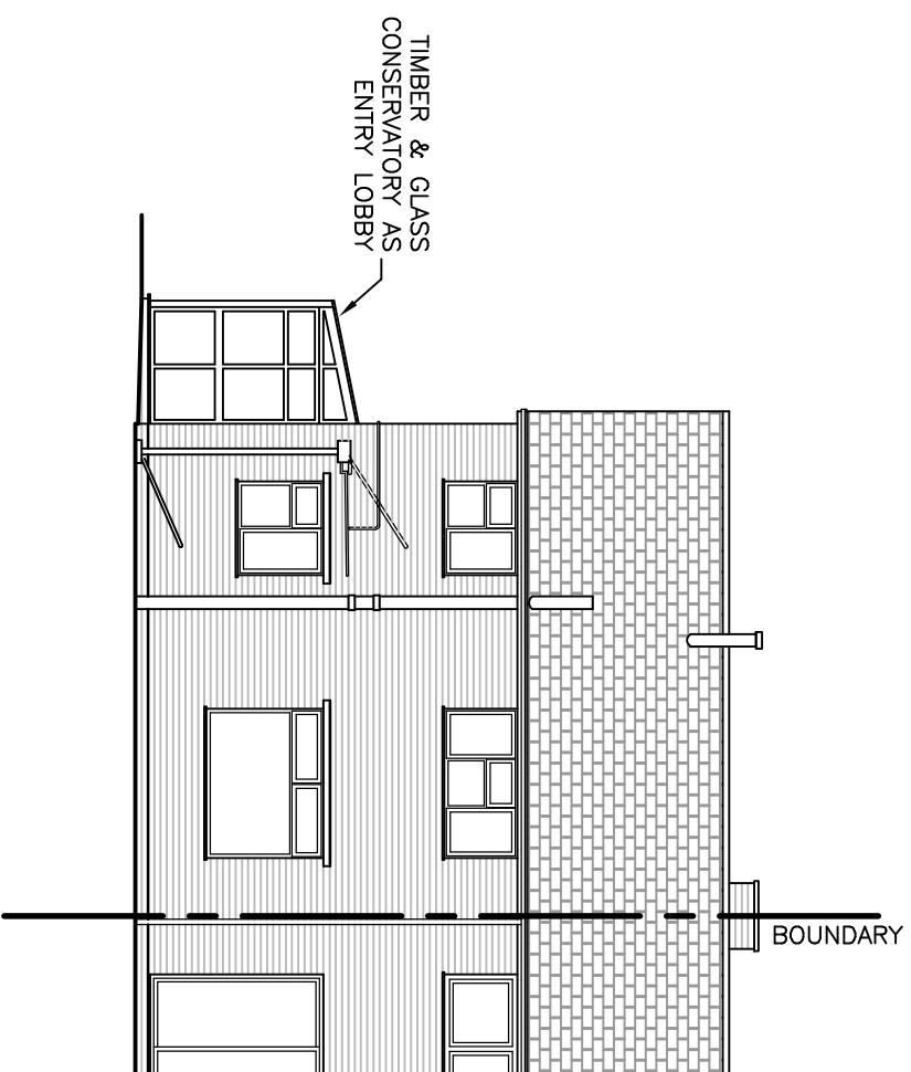
REAR ELEVATION (1:100)
