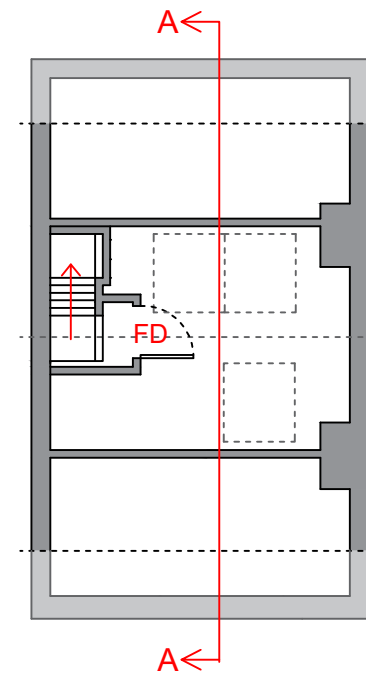
Proposed loft floor plan
