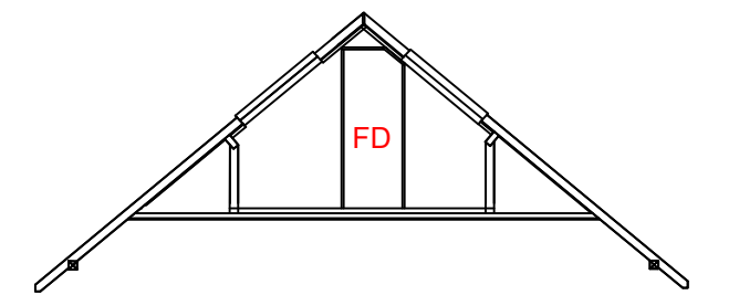
Proposed roof section A-A
