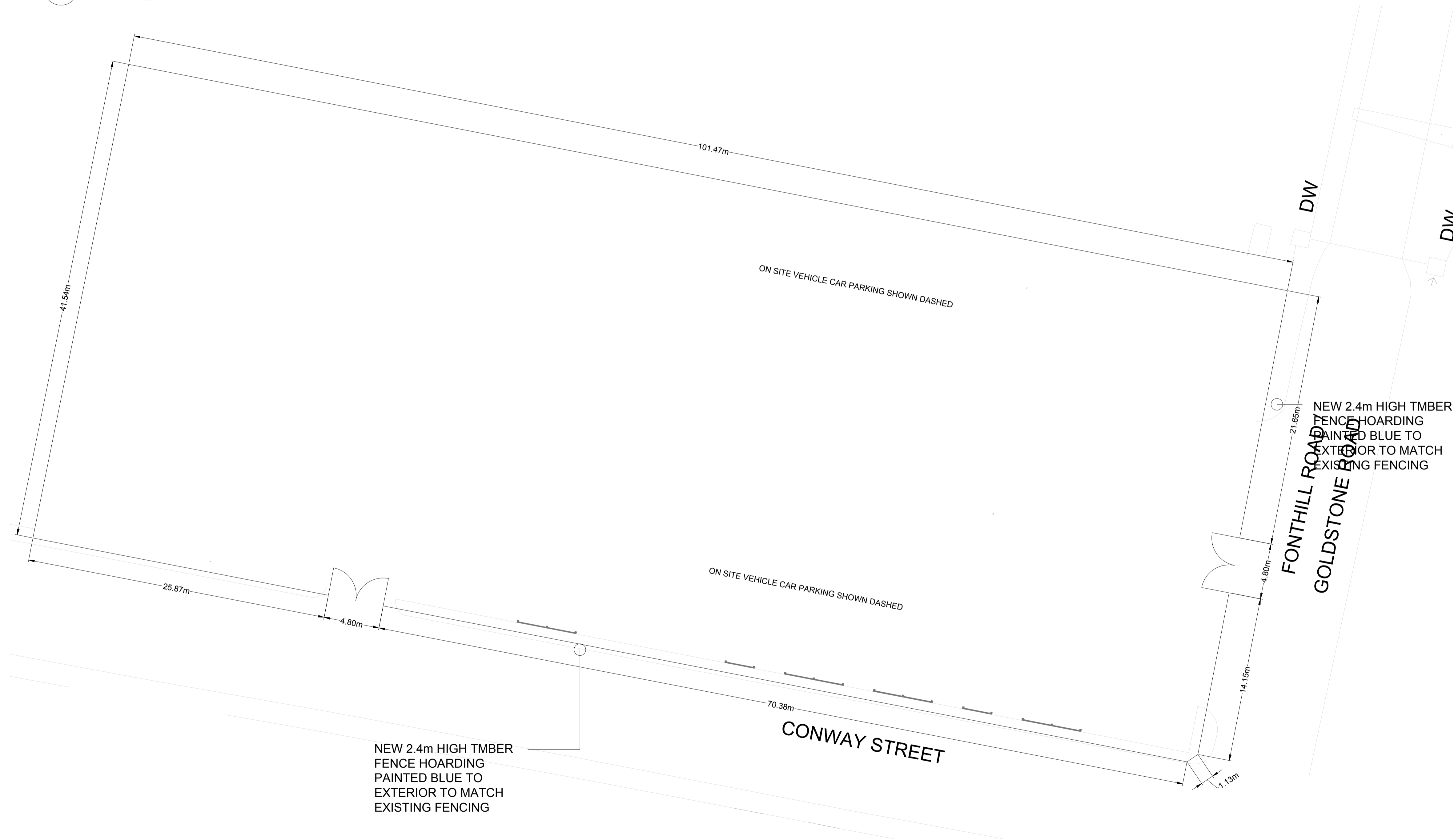
2 106 1:200 HOARDING LAYOUT PROPOSED
