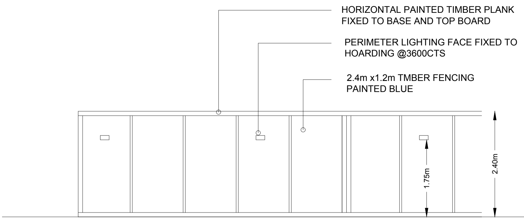
1 106 1:50 TYPICAL HOARDING ELEVATION PROPOSED
