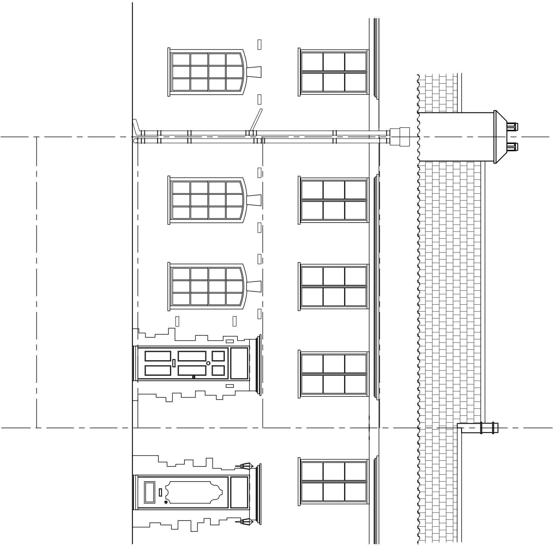
Front Elevation
