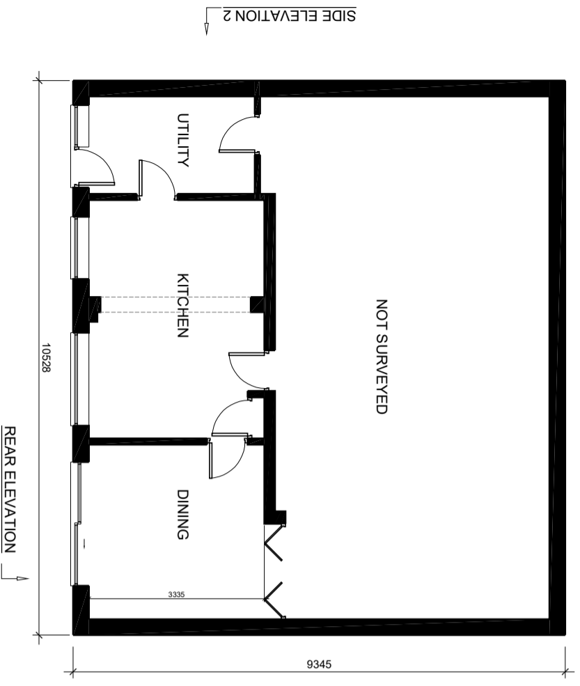
GROUND FLOOR PLAN AS EXISTING
