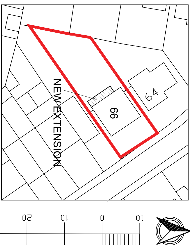
BLOCK PLAN 1:500
