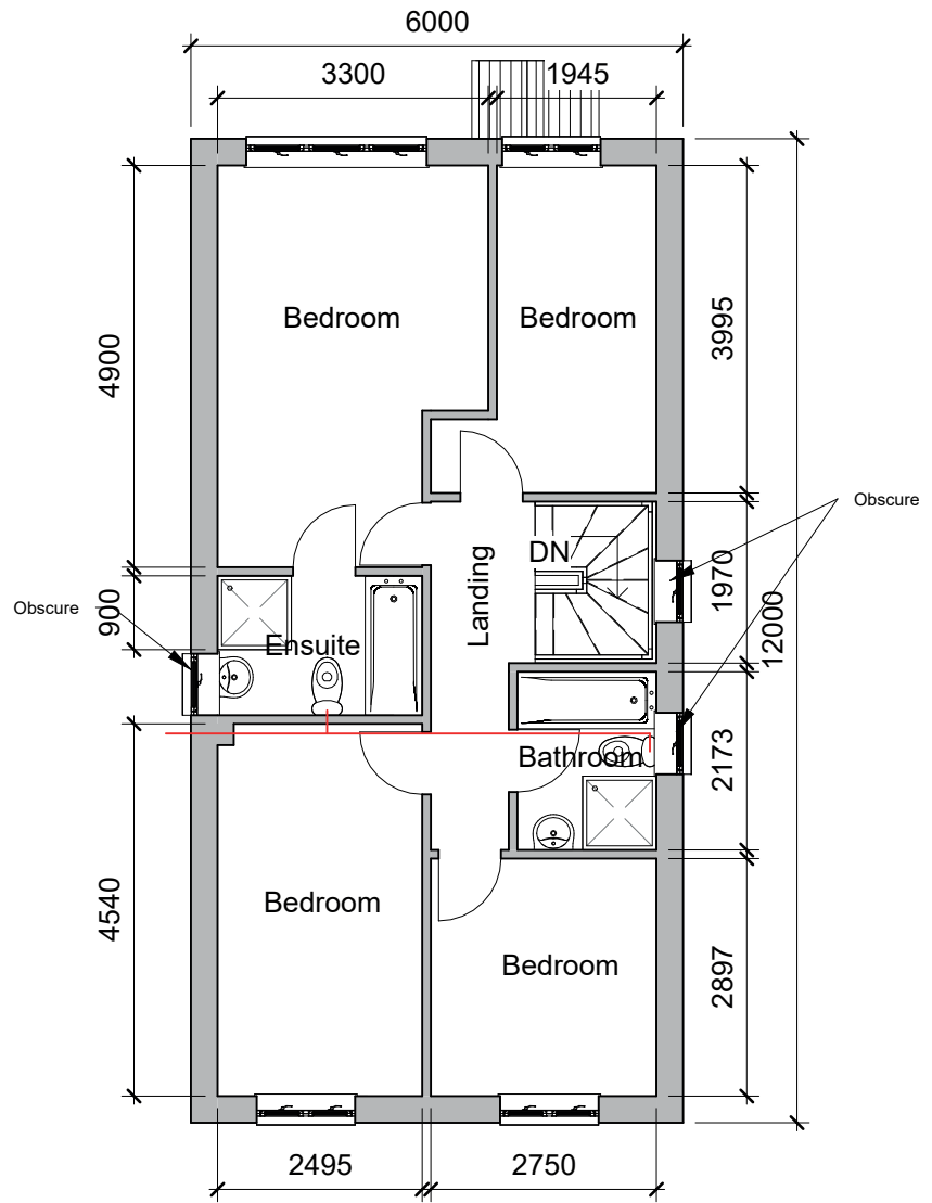
2 First Floor Drain Plan 1 : 100
