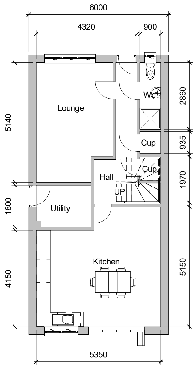
1 Ground Floor 1 : 100
