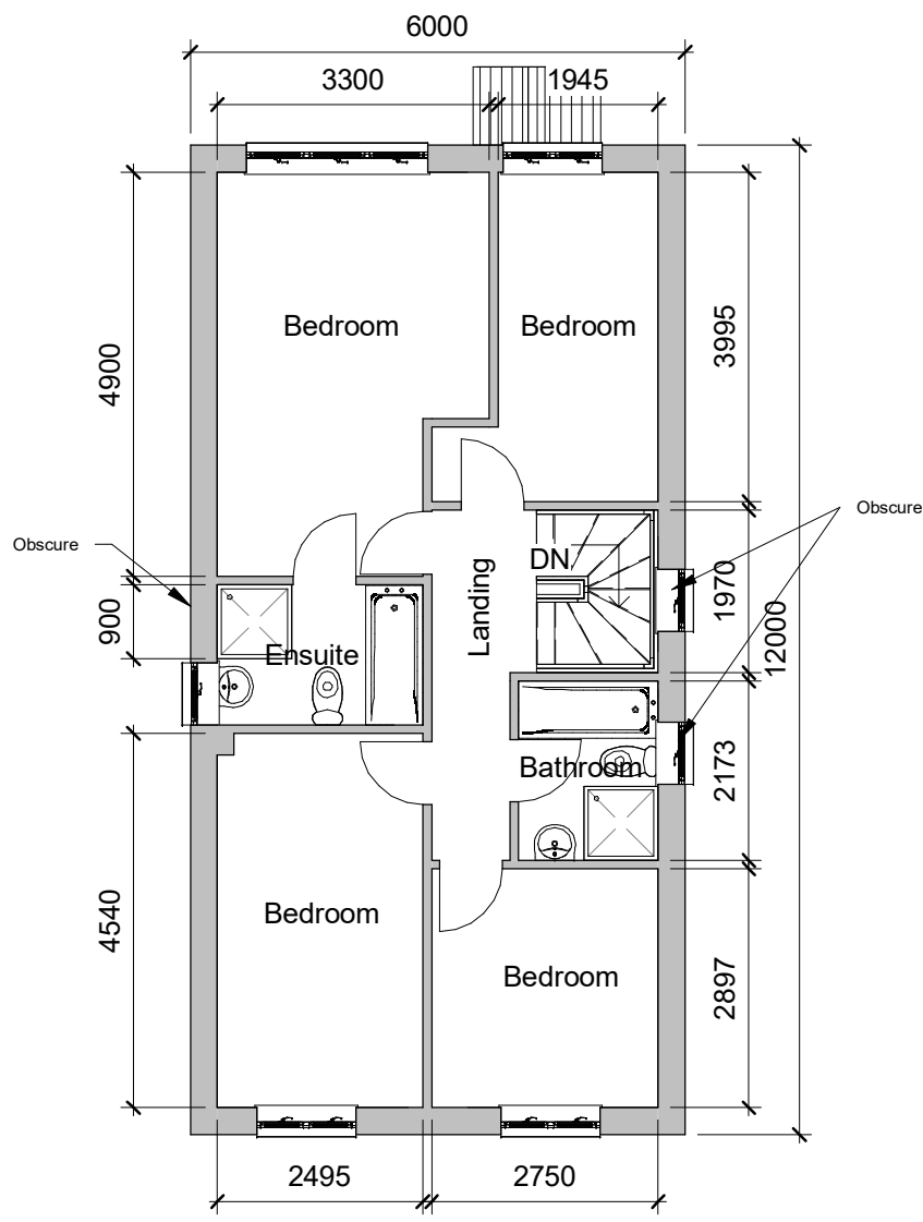
2 First Floor 1 : 100
