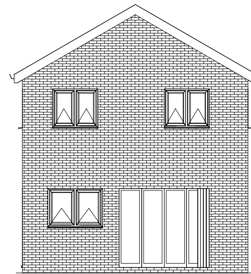
3 Rear Elevation 1 : 100
