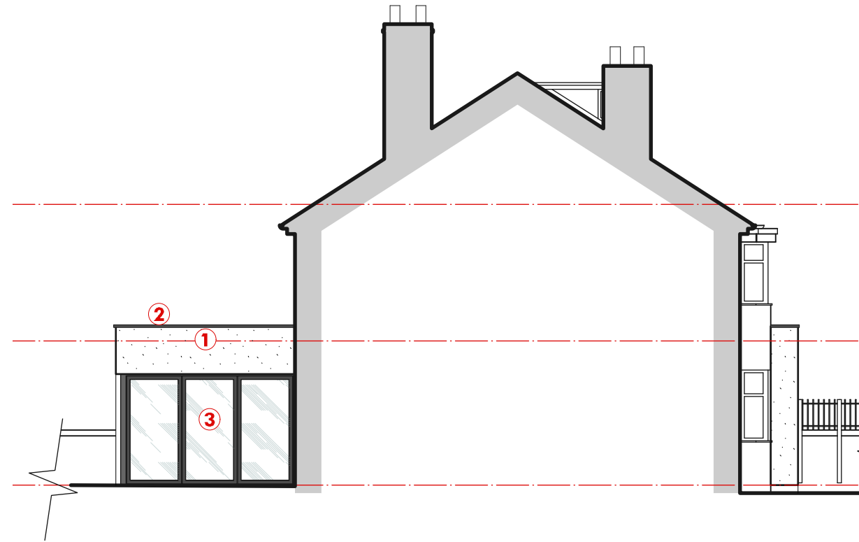
gable elevation
