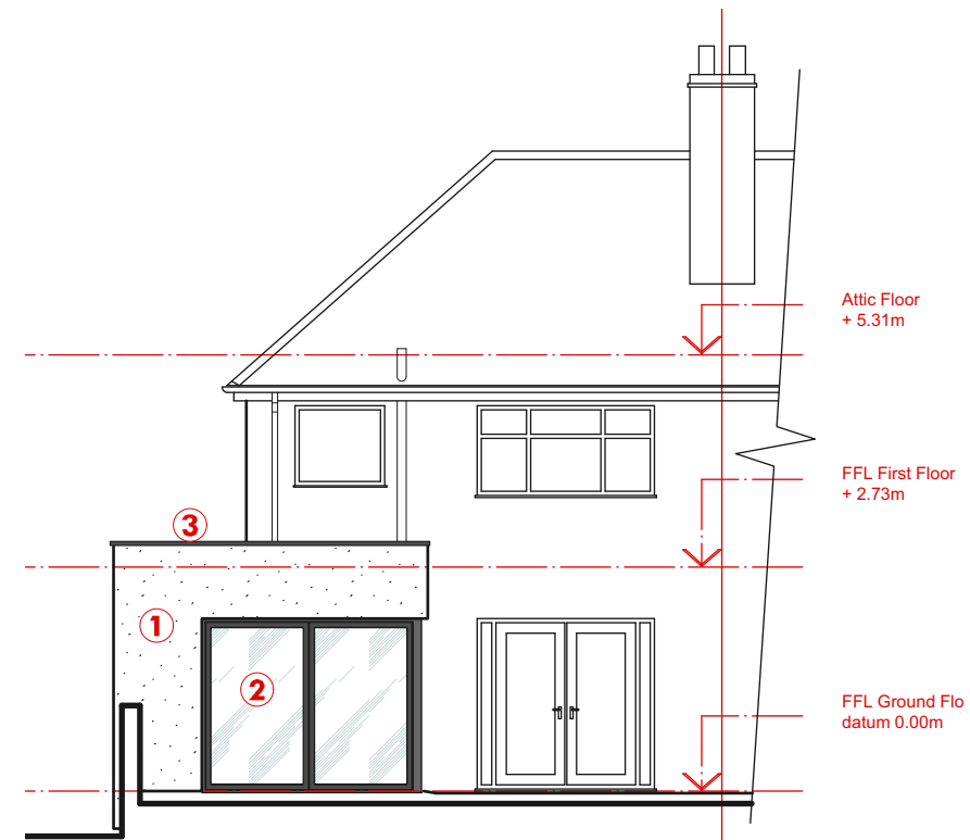
rear elevation
