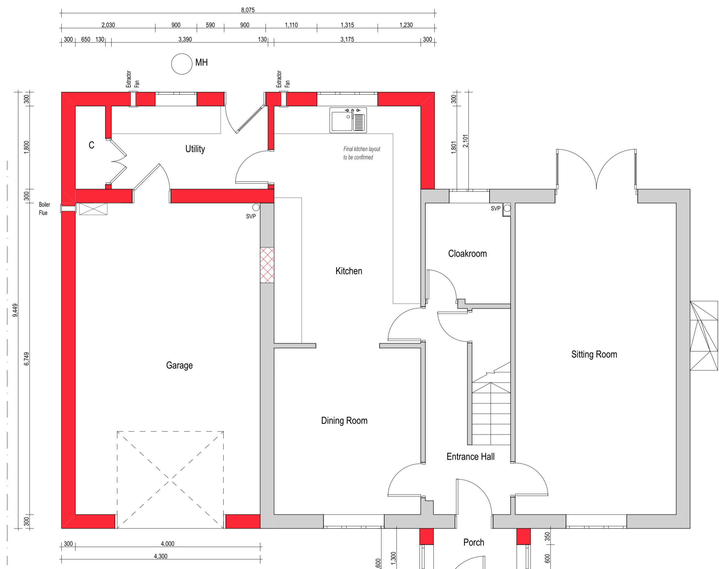
Proposed GF Layout Scale: 1:50
