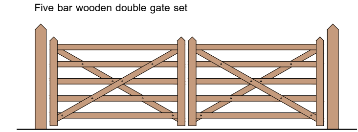
Elevation 1:50 Showing proposed residential gated entrance
