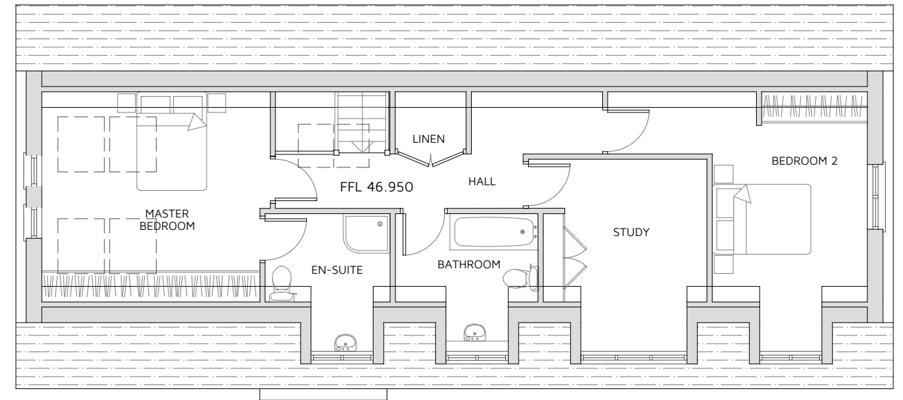
Proposed First Floor Plan 1:100 @ A3
