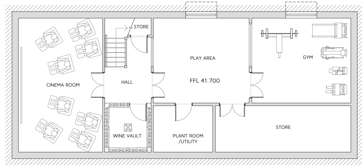
Proposed Basement Plan 1:100 @ A3
