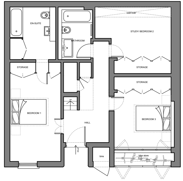
1 03 GROUND FLOOR PLAN
