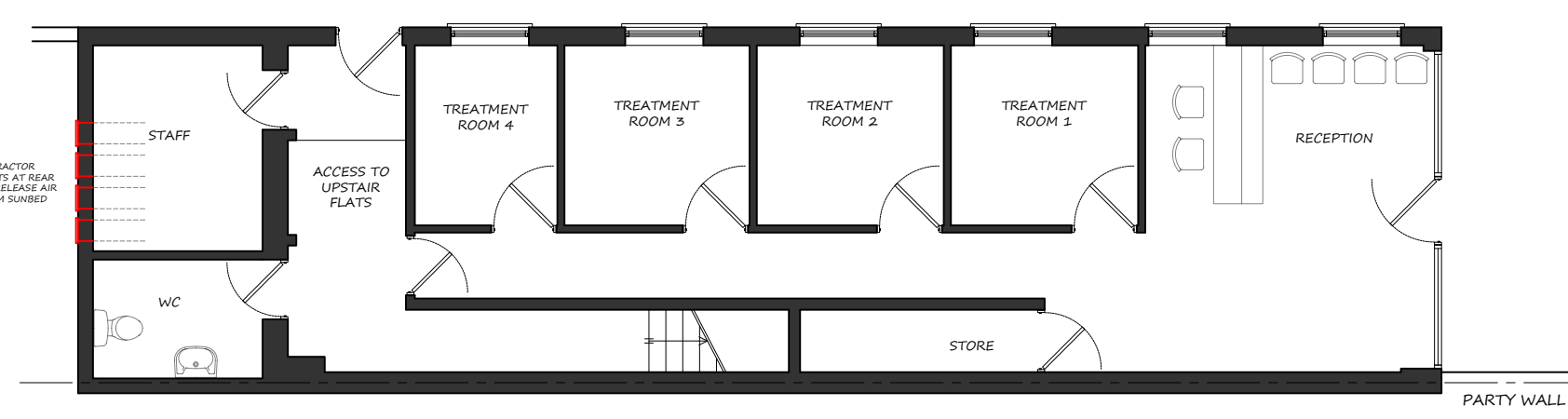
PROPOSED GROUND FLOOR PLAN 1:100
