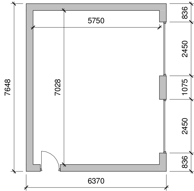
1 20 Ground Floor 1 : 100
