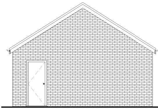
4 South Elevation 1 : 100
