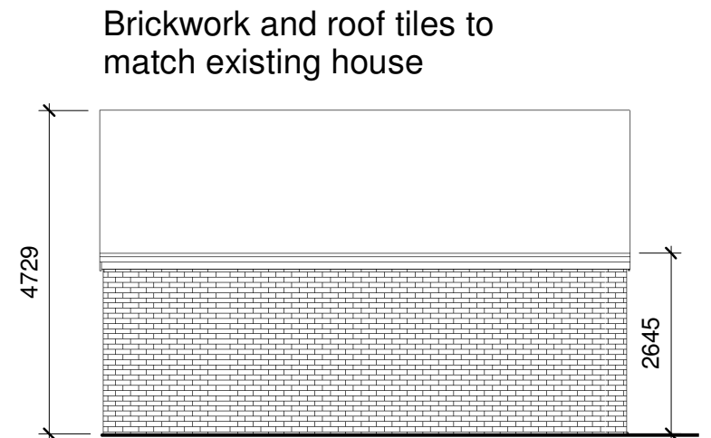
5 West Elevation 1 : 100
