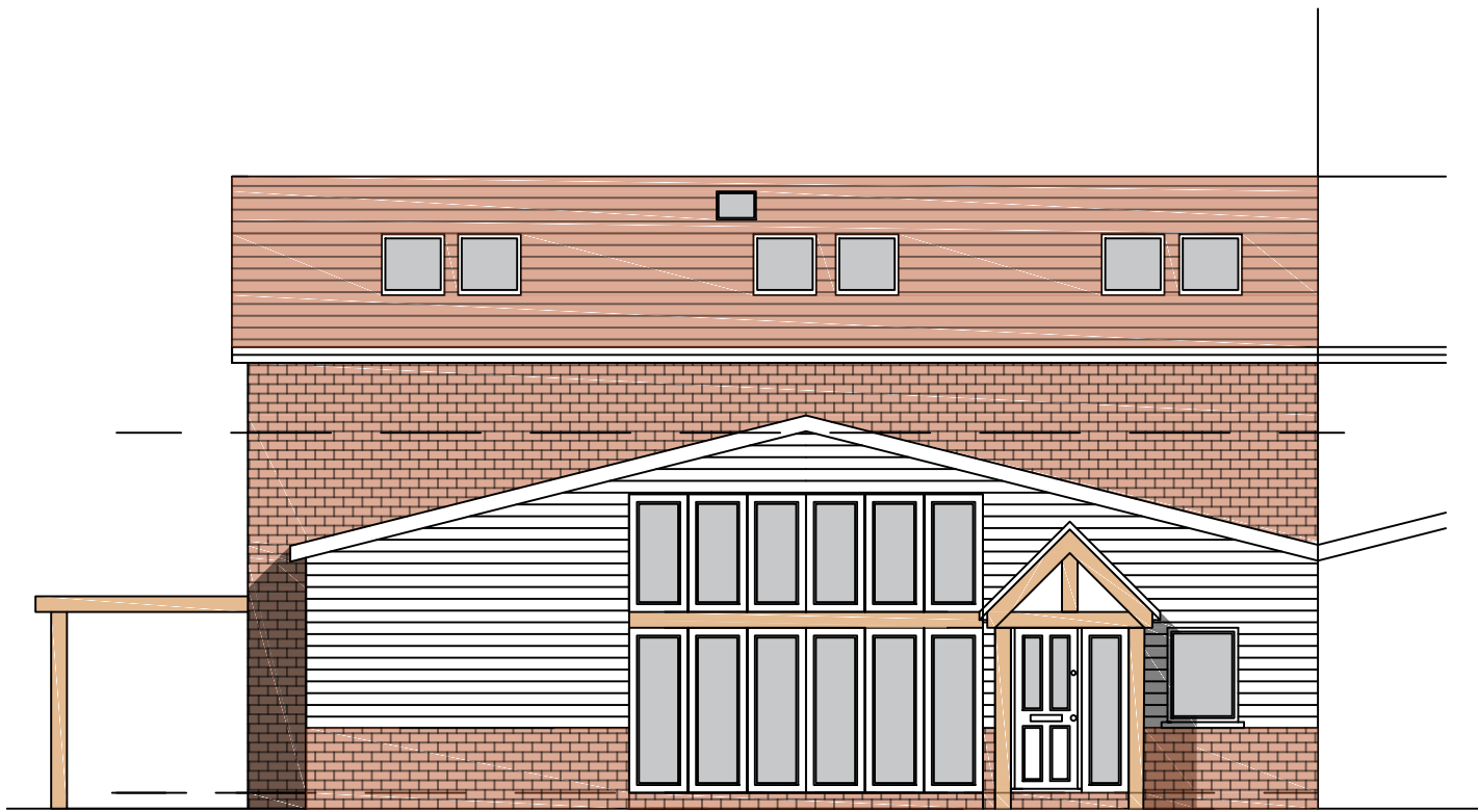
South Elevation
