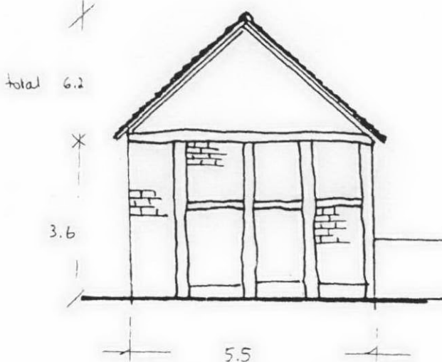
NORTH ELEVATION
