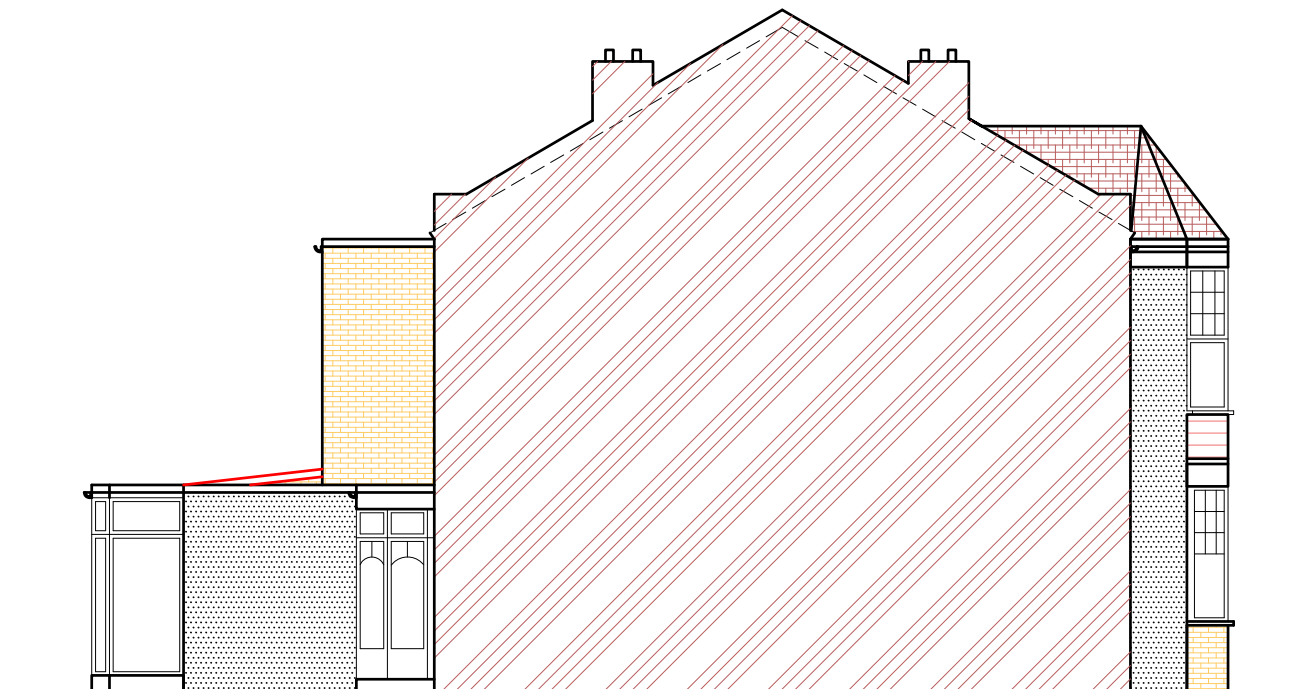
Proposed Side Elevation - B
