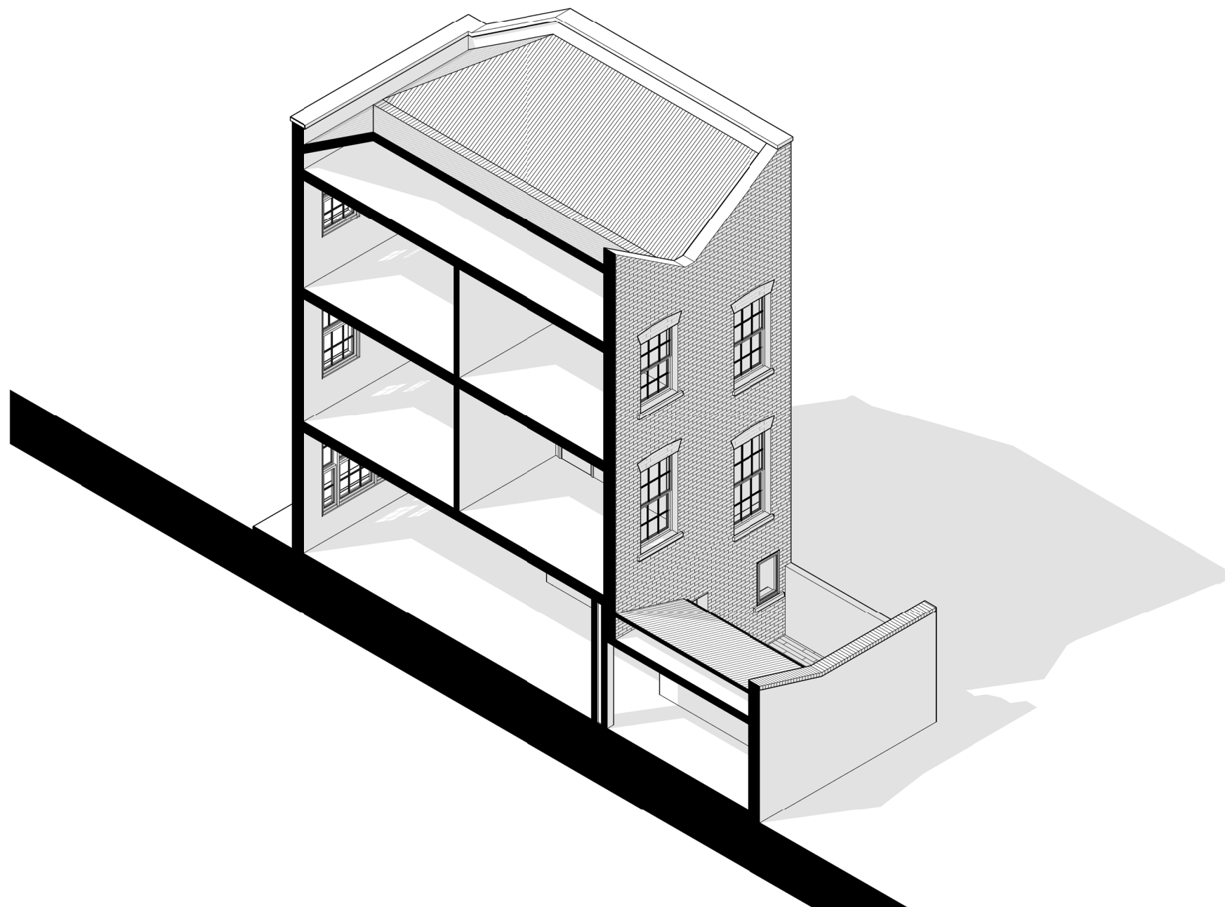
3D SECTION
