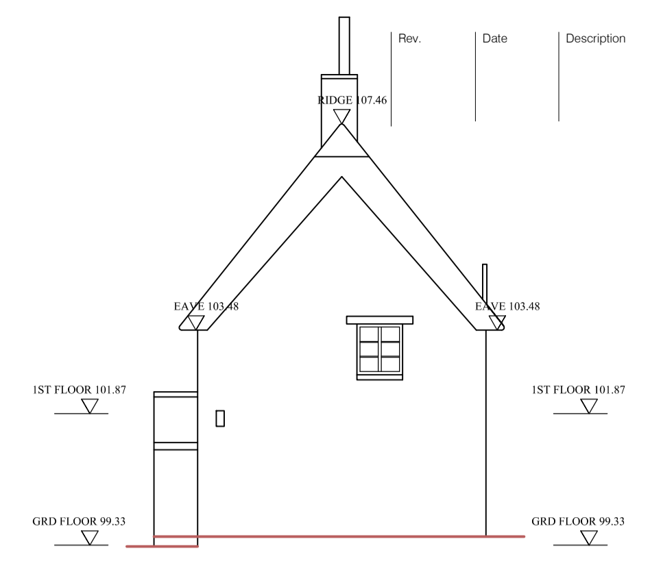
NORTH ELEVATION 1:100
