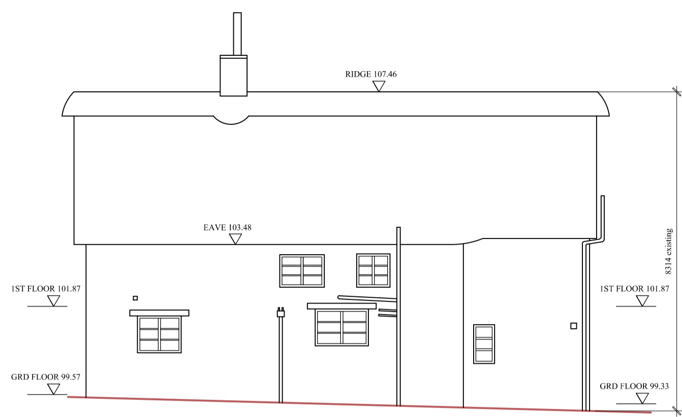
WEST ELEVATION 1:100
