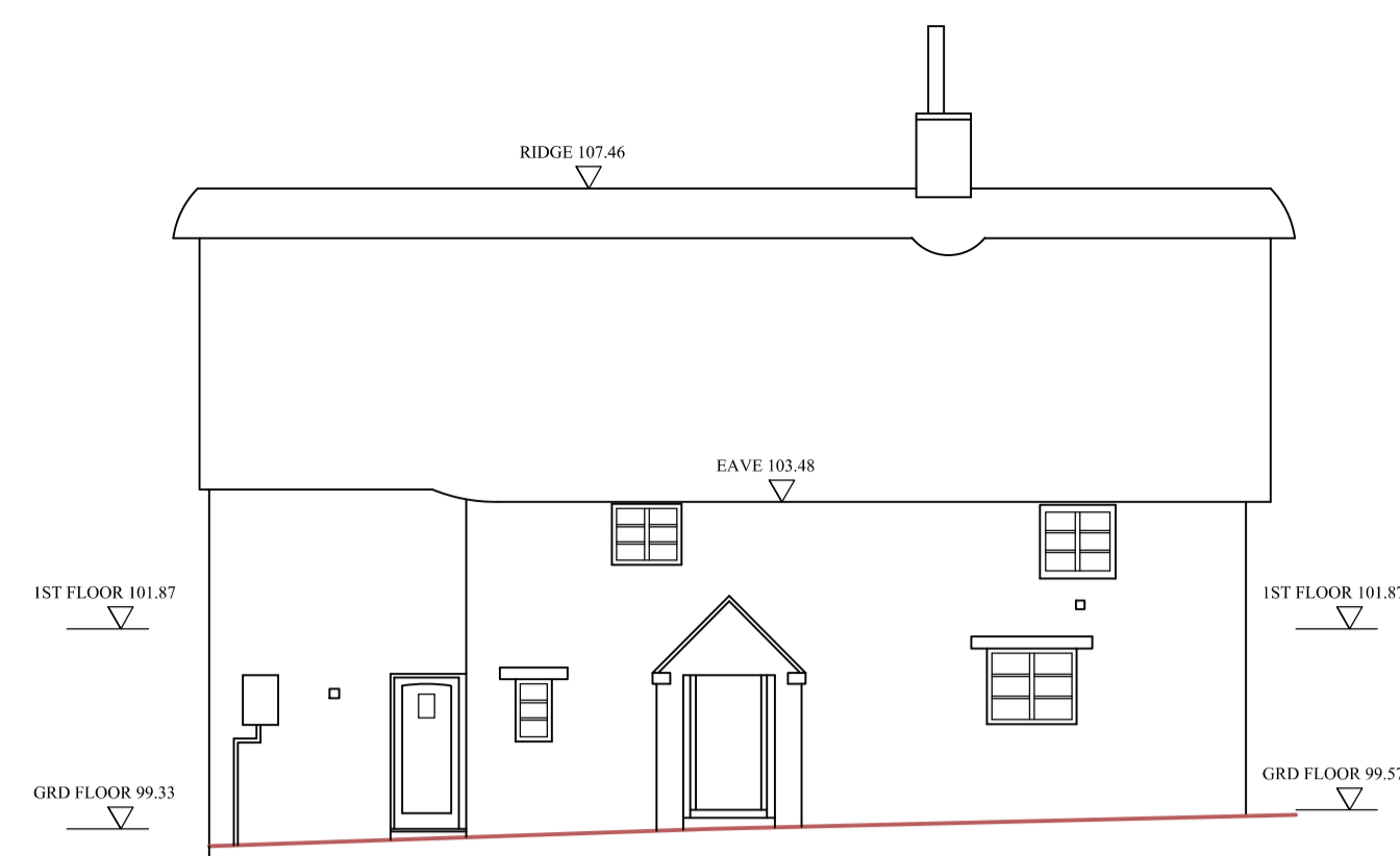
EAST ELEVATION 1:100
