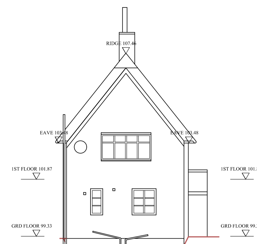
SOUTH ELEVATION 1:100
