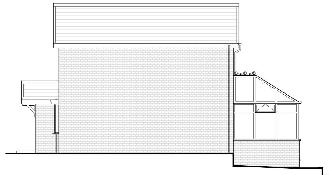
SIDE ELEVATION (NORTH-EAST FACING)
