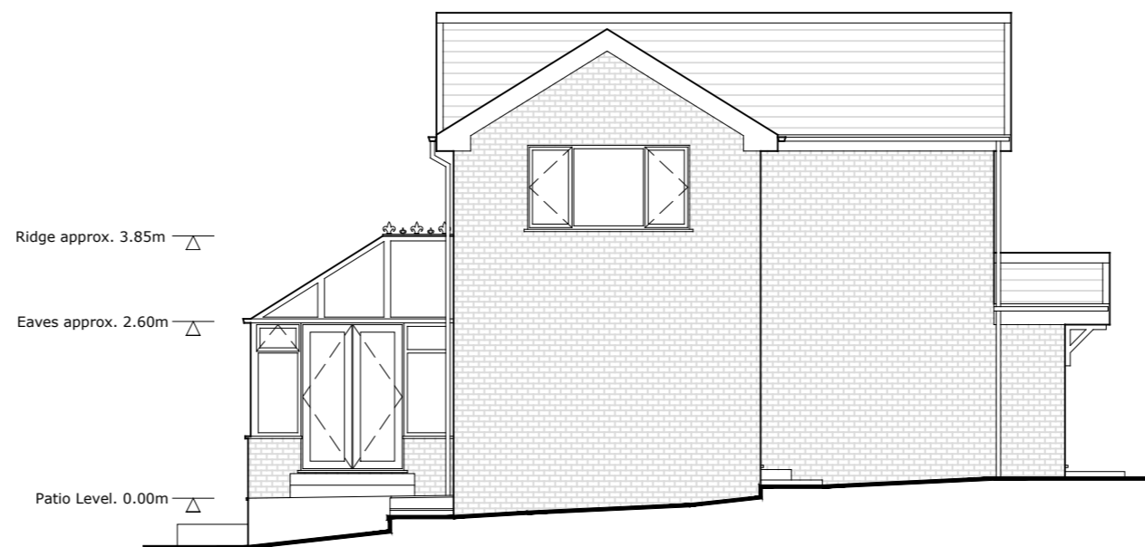
SIDE ELEVATION (SOUTH-WEST FACING)
