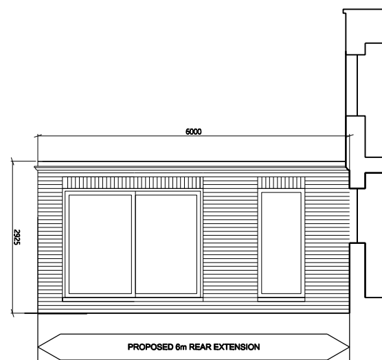
PROPOSED EXTENSION SIDE ELEVATION
