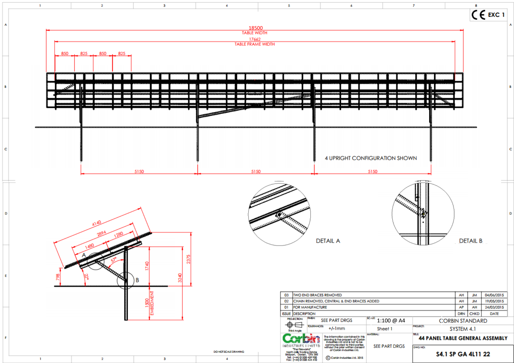
Example of a 44 panel array mounting kit: capable of mounting 4 x 11 solar PV modules
