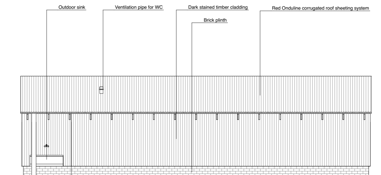
4 Classroom South Elevation 1:100
