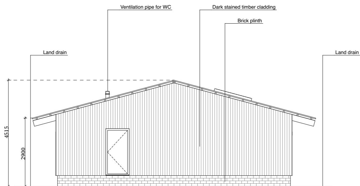
1 Classroom East Elevation 1:100
