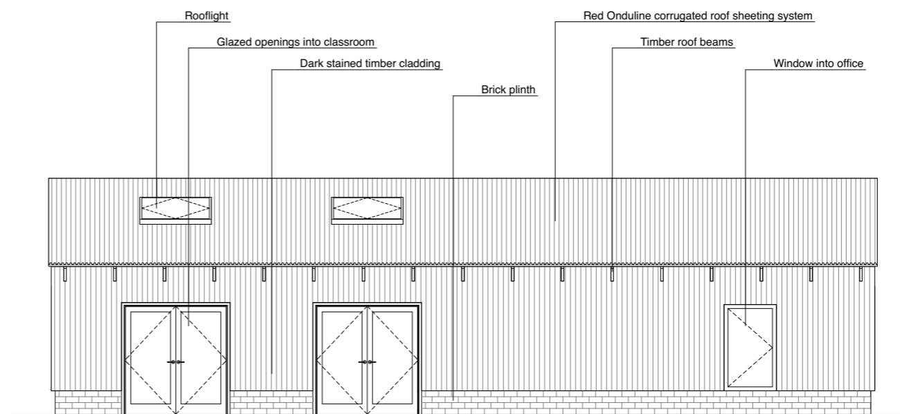
2 Classroom North Elevation 1:100
