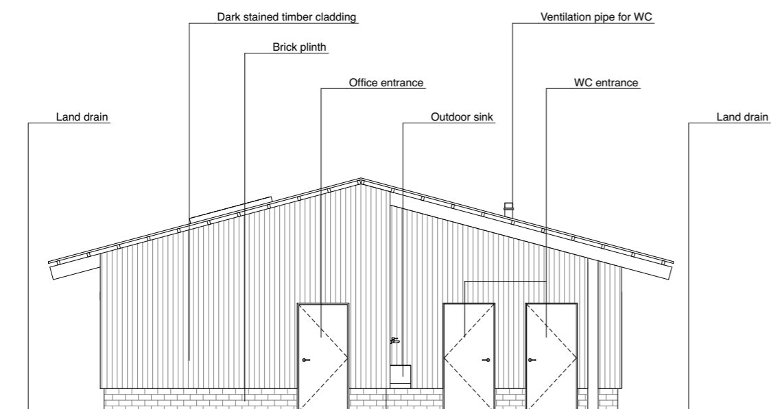
3 Classroom West Elevation 1:100
