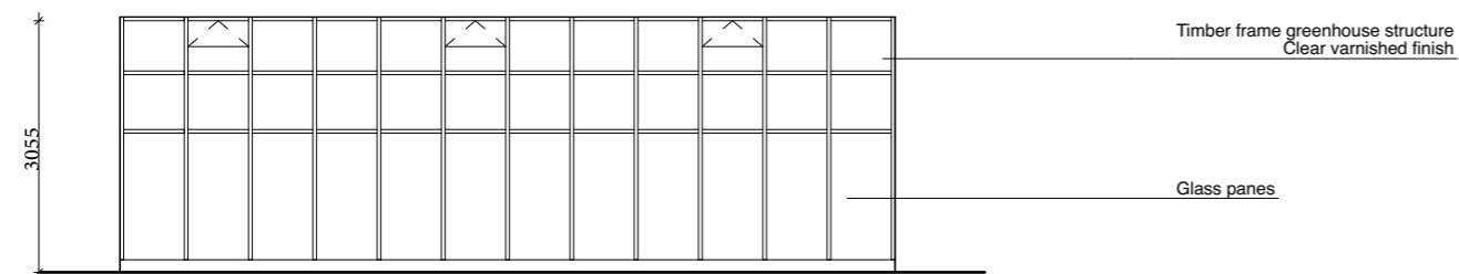
2 Greenhouse South Elevation 1:100
