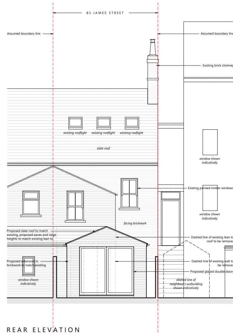
REAR ELEVATION
