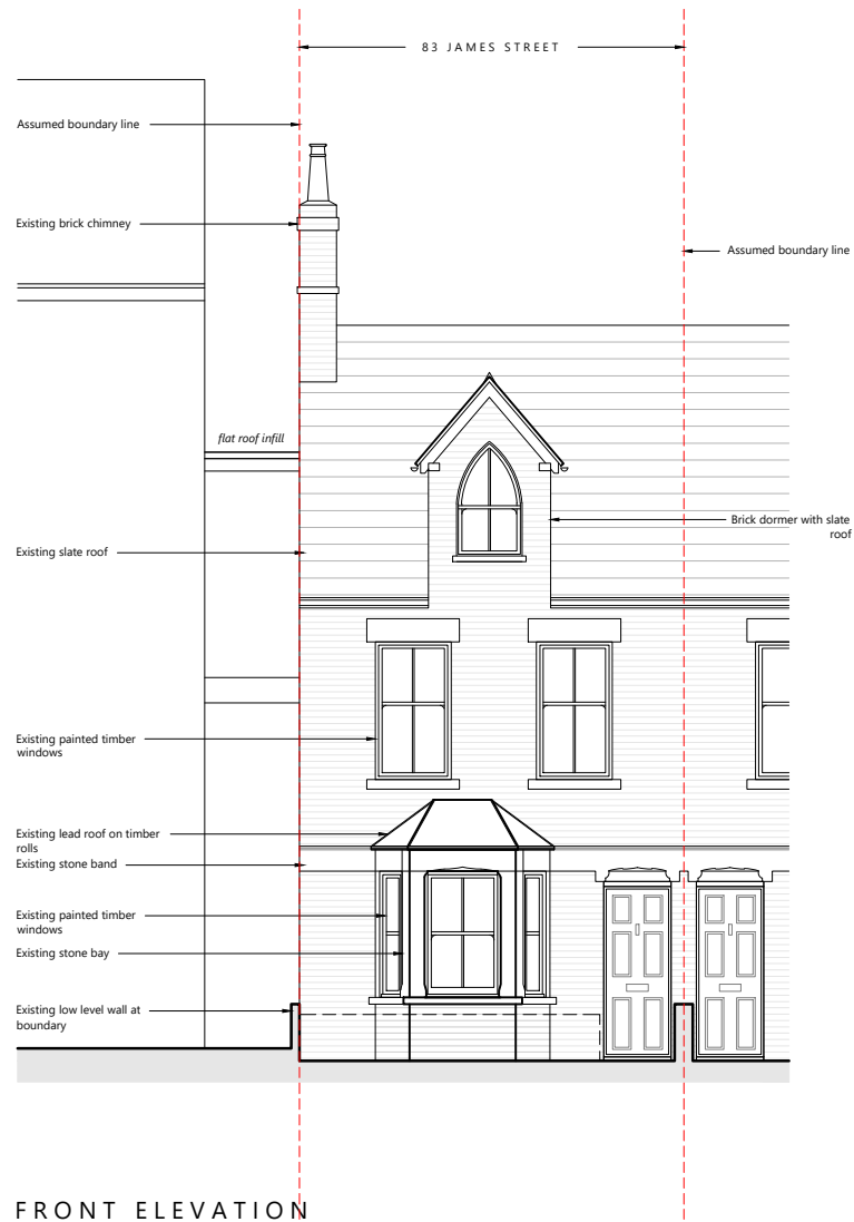
FRONT ELEVATION
