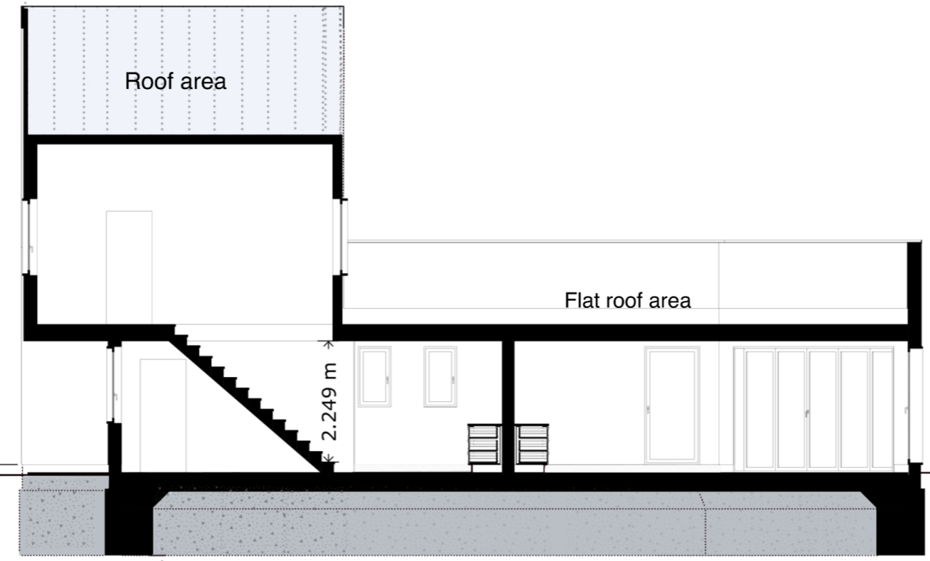
Section E2, Drawing PLNG / 02 / 10 A
