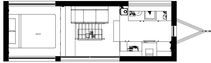
LOFT FLOOR PLAN
