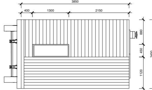
ELEVATION NORTH
