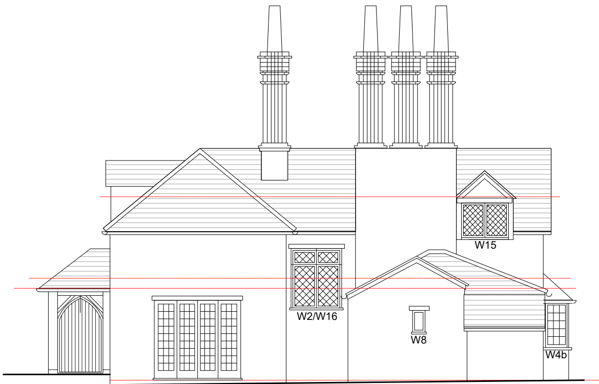
EAST ELEVATION
