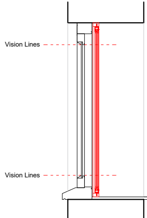
VERTICAL SECTION
