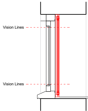
VERTICAL SECTION
