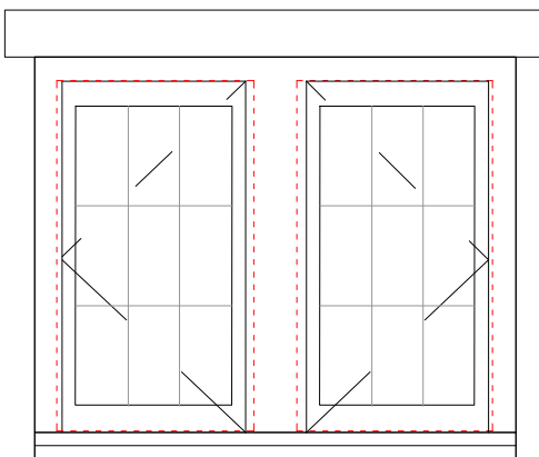
EXTERNAL ELEVATION
