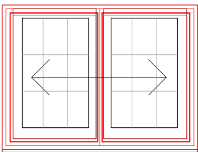
INTERNAL ELEVATION
