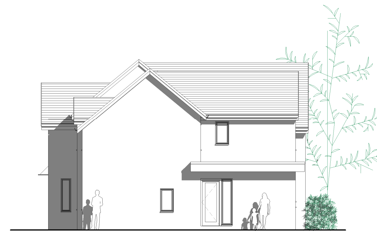
4 Side Elevation 2 1 : 100
