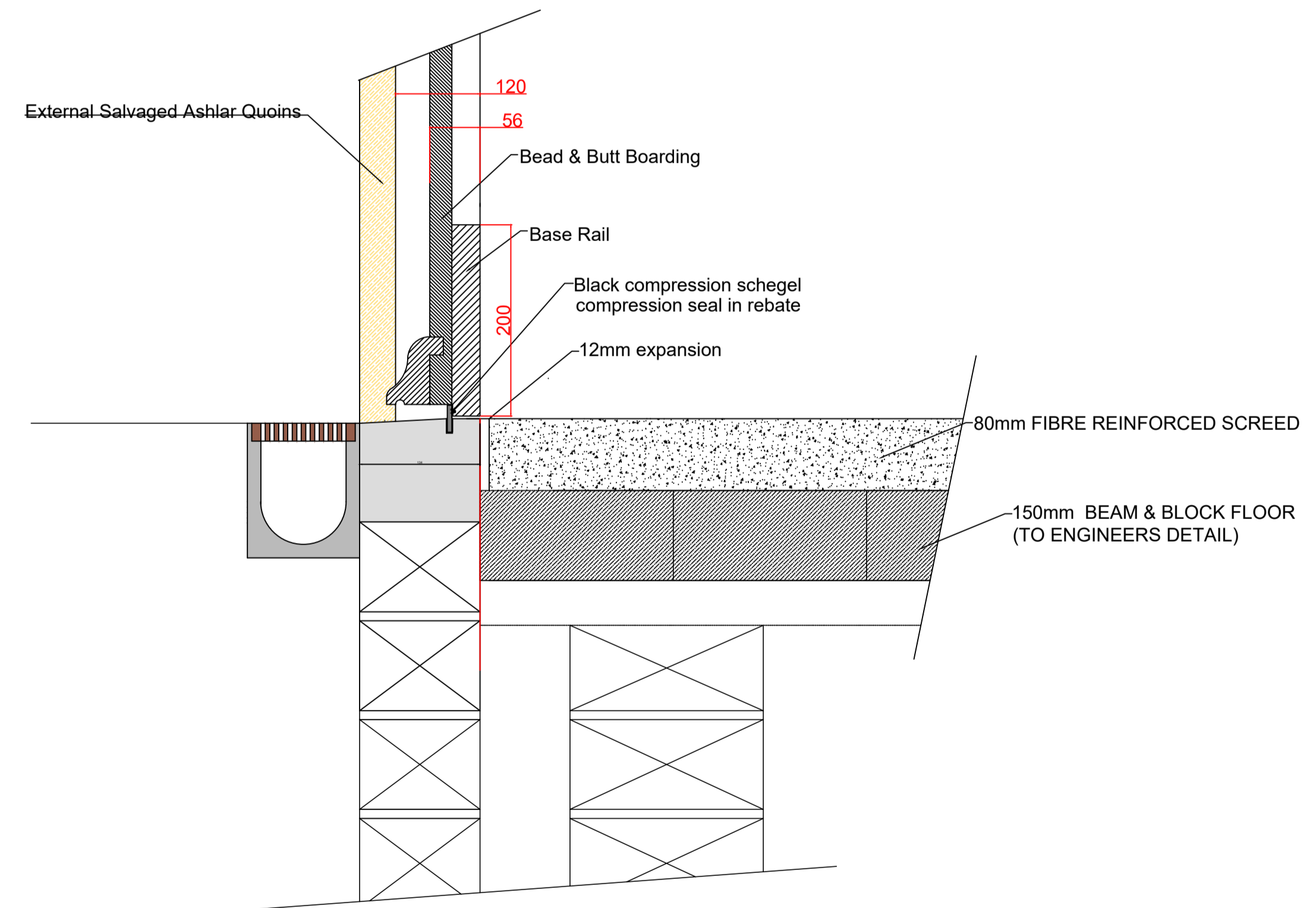
D-D TYPICAL GARAGE DOOR CILL DETAIL
