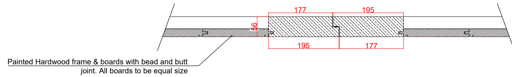
B-B MEETING SYTLE SECTION
