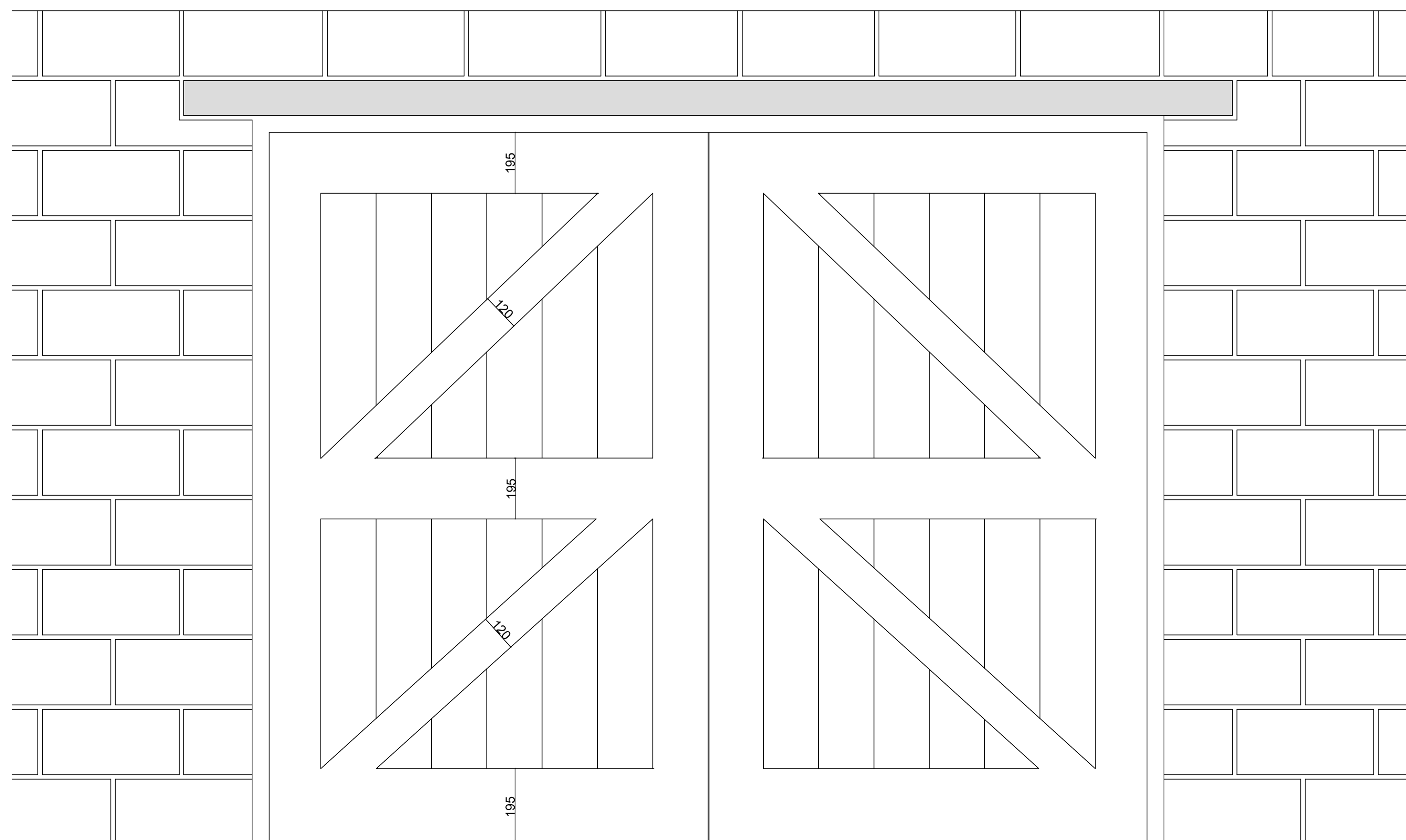
PAINTED GARAGE DOORS & FRAME WITH HOOKS AND BAND HINGE EXTERNAL VIEW & INTERNAL VIEW - BUILDINGS C & D
