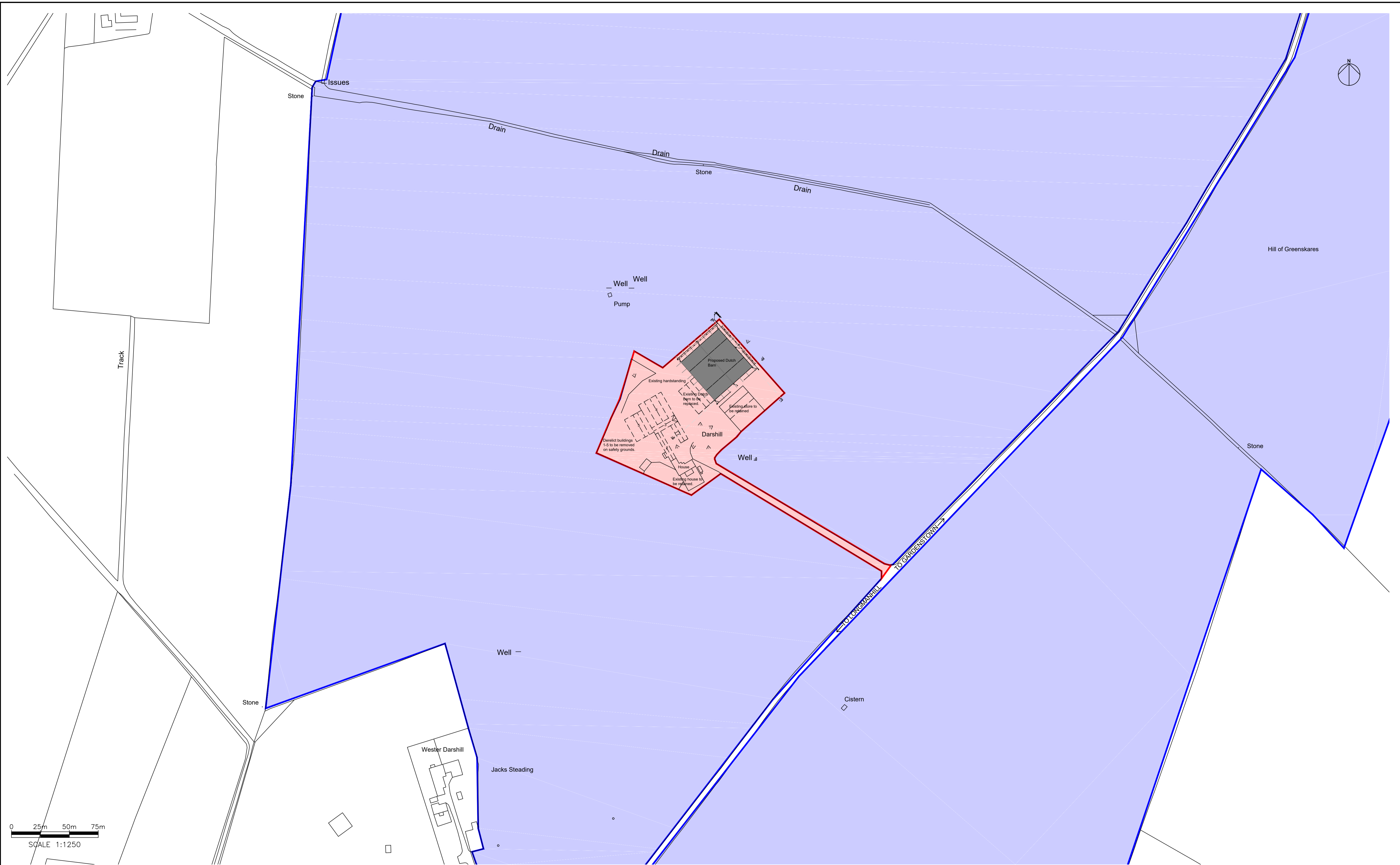
LOCATION PLAN SCALE 1:1250
