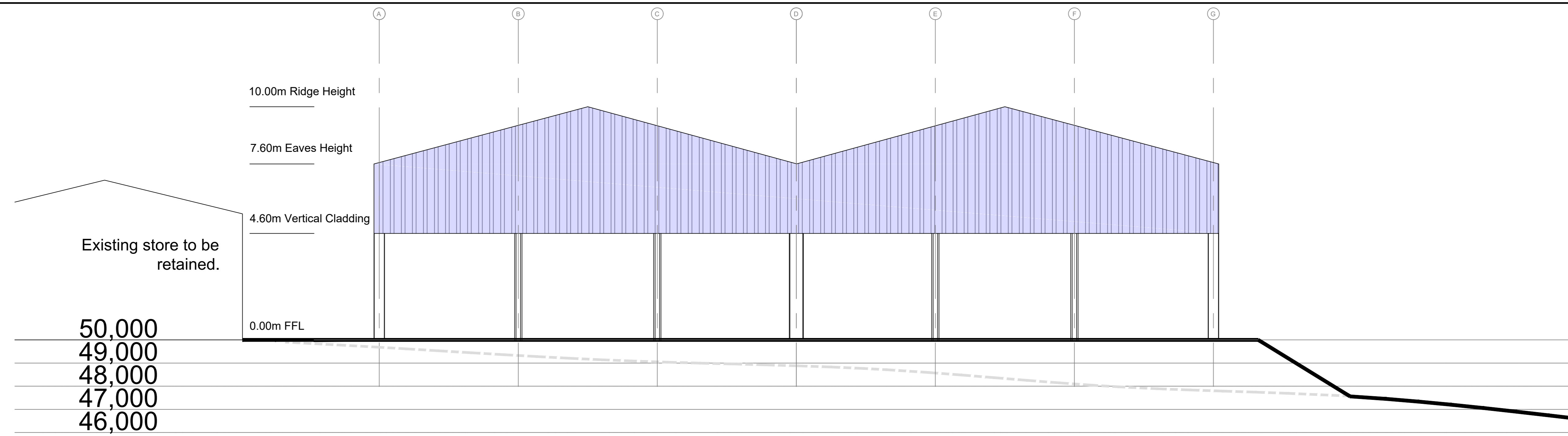
NORTH EAST ELEVATION
