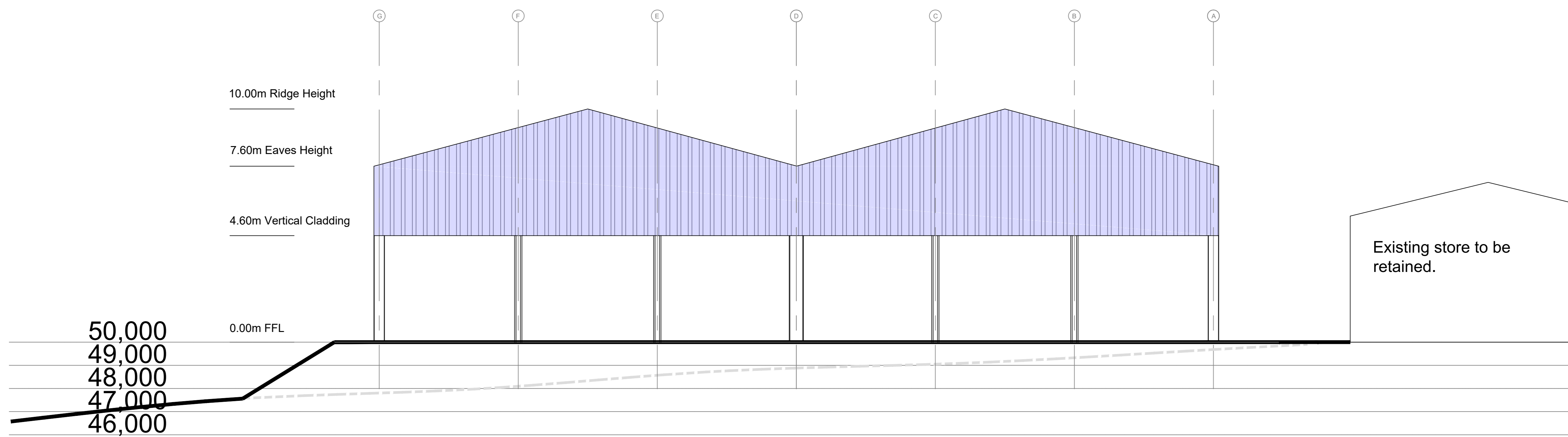
SOUTH WEST ELEVATION
