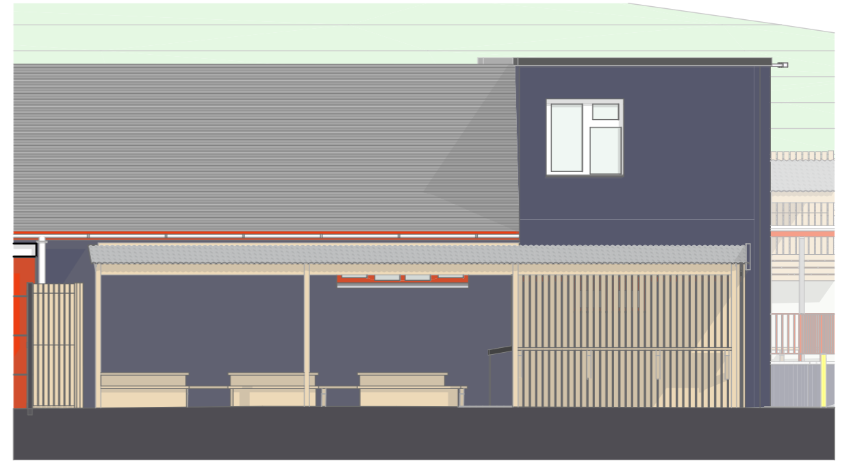
Section S3.2 1:100
